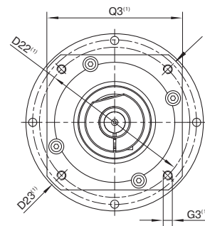
Drawing corresponds to a PSFN090 / 1-stage / flange output shaft / 14 mm clamping system / motor adaptation - 2-part - round universal flange / B5 flange type motor
