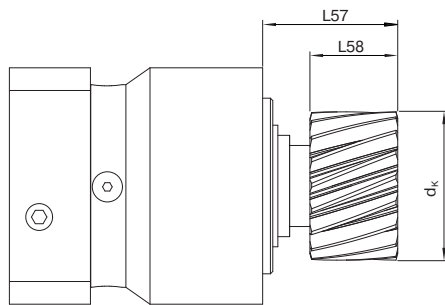
PLPE 带小齿轮 PLPE with pinion
